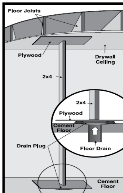
Figure 11. Drain plug bracing.
