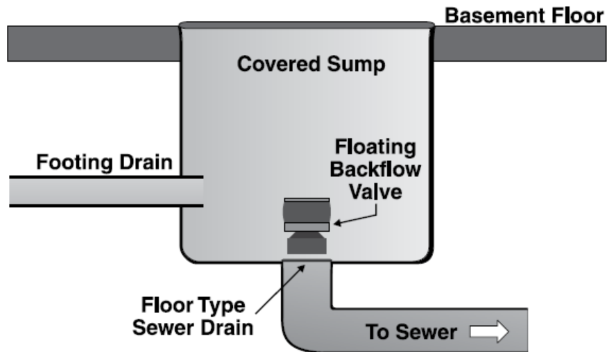
Figure 20. Footing drain.
